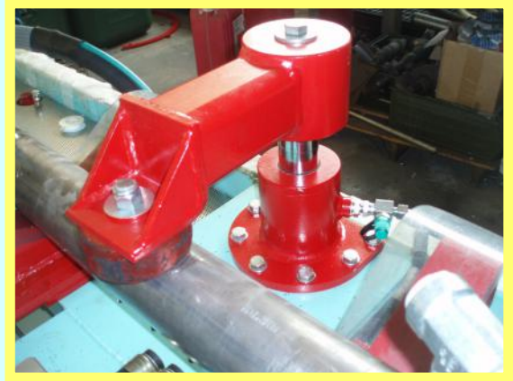
Cylinder locking system with pulling hydraulic cylinder. ACSTT0000030
